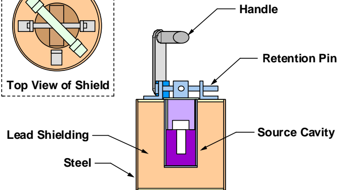
Cross Section of Shield
